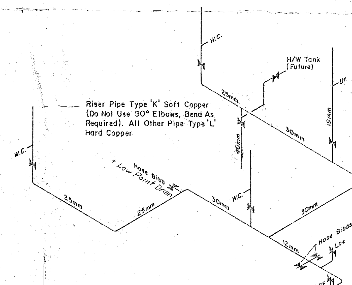
WATER DISTRIBUTION ISOMETRIC
