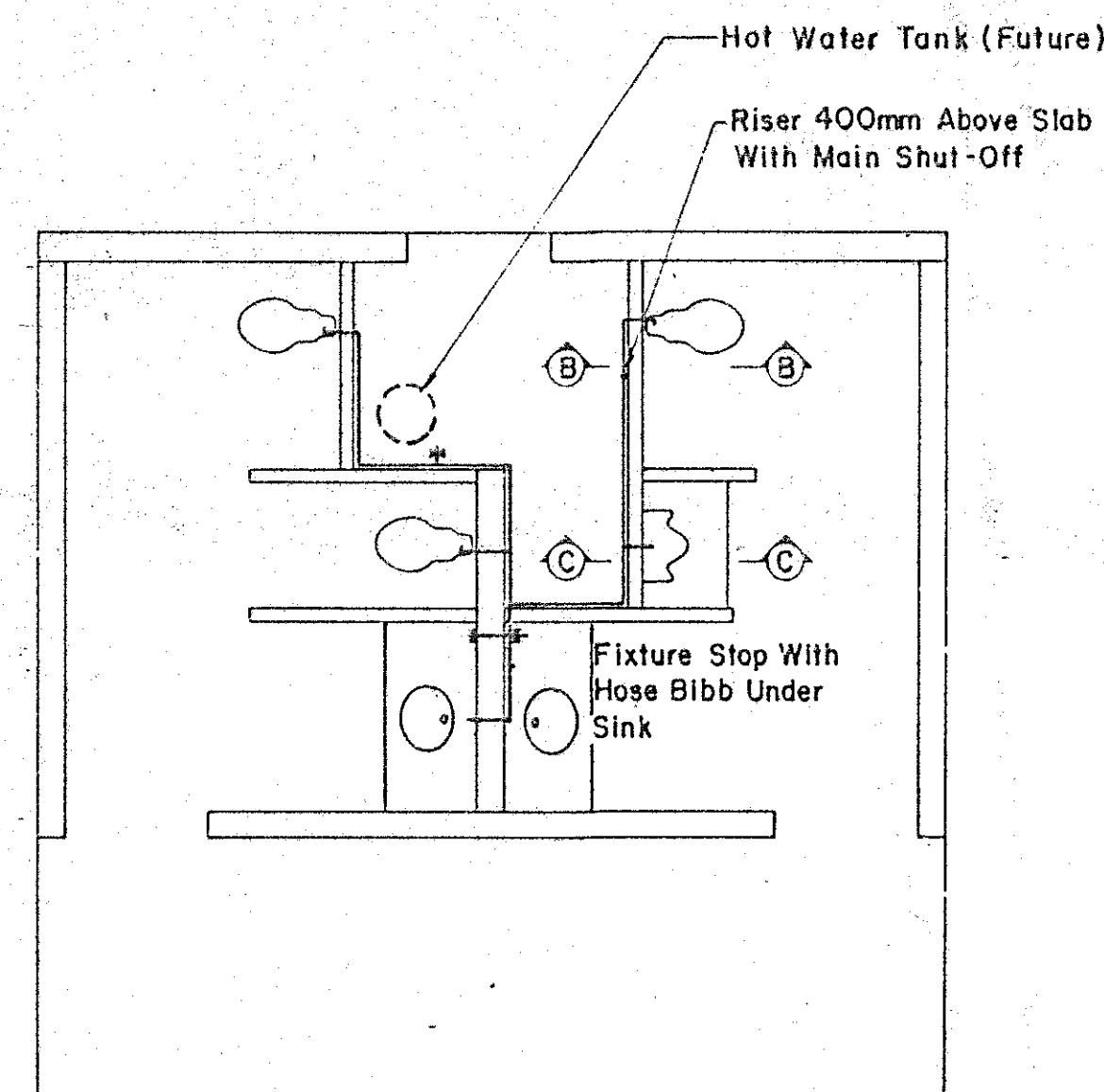
PLUMBING LAYOUT
