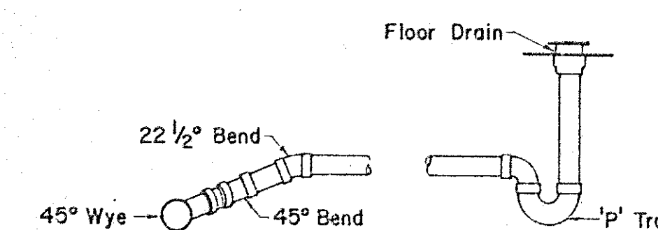
FLOOR DRAIN DETAIL
