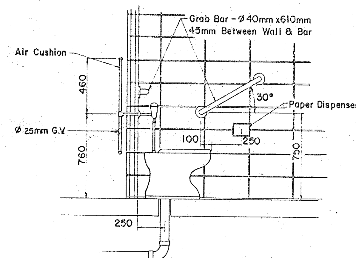
SECTION - B-B
