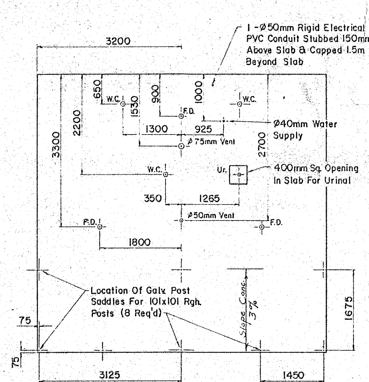
SLAB PLAN
