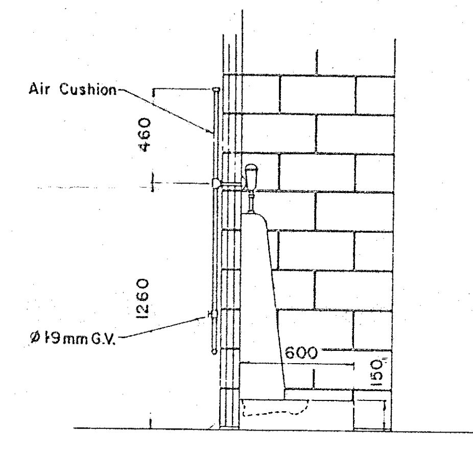
SECTION C-C
